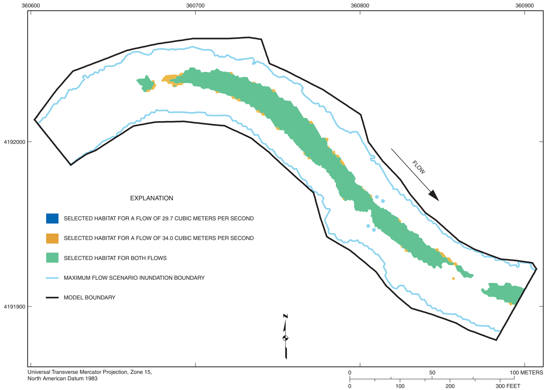
Figure 1-19. Selected habitat area distribution for habitat category 7 (paddlefish) at flows of 29.7 and 34.0 cubic meters per second at Marmaton River site M1.
